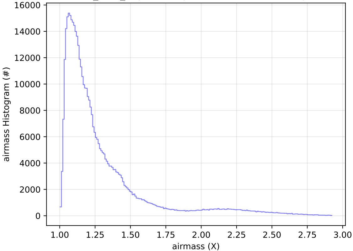
noroll_v3.4_10yrs All sky z band: airmass Histogram
