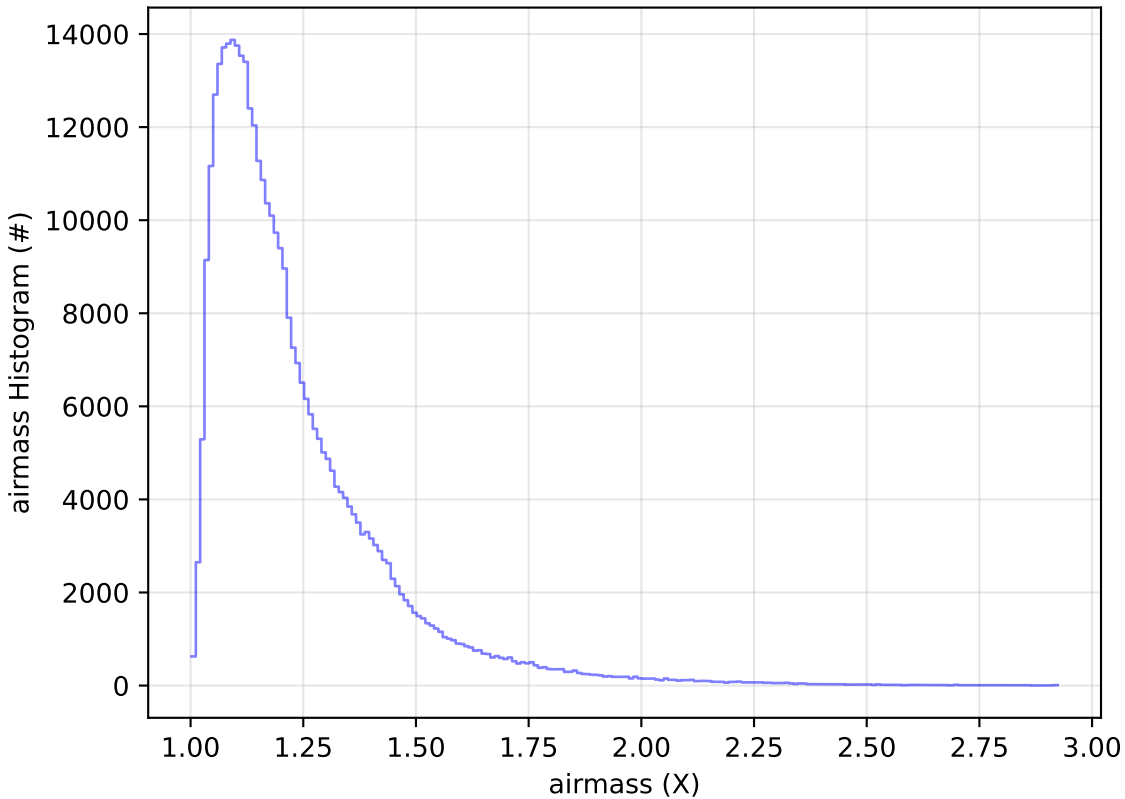
noroll_v3.4_10yrs All sky y band: airmass Histogram
