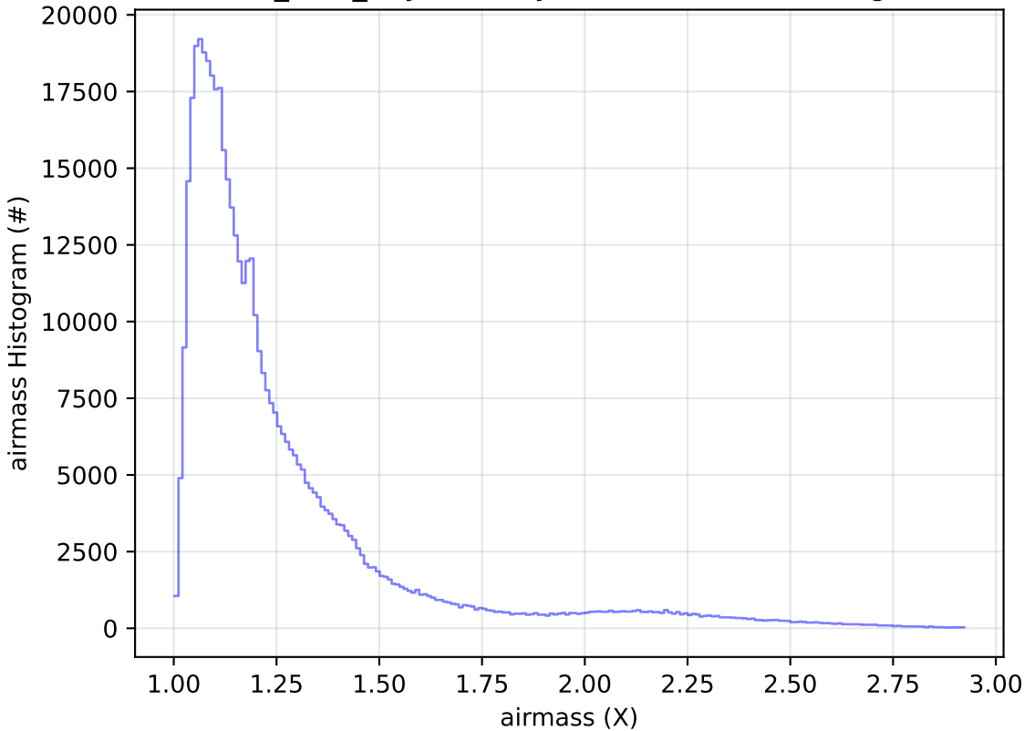
noroll_v3.4_10yrs All sky i band: airmass Histogram
