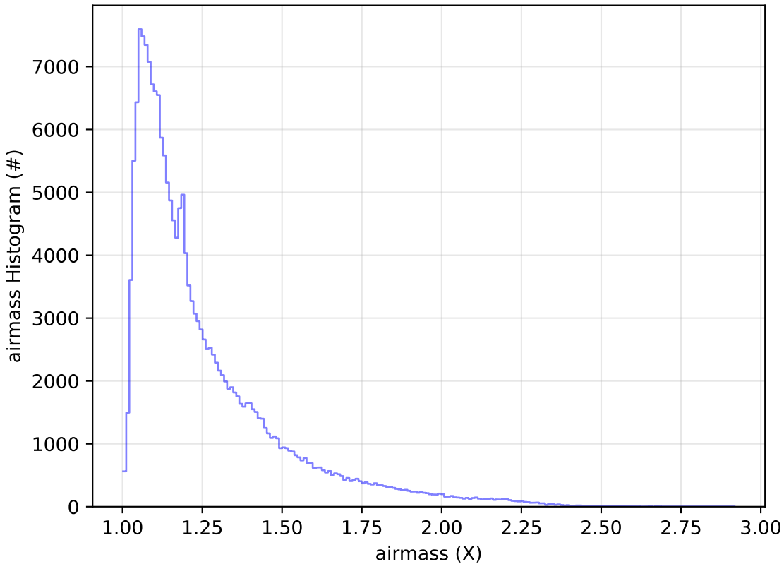
noroll_v3.4_10yrs All sky g band: airmass Histogram
