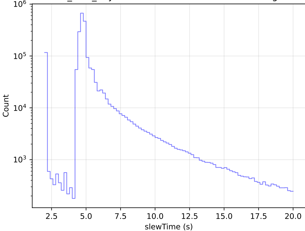
noroll_v3.4_10yrs All visits: Zoom Slew Time Histogram
