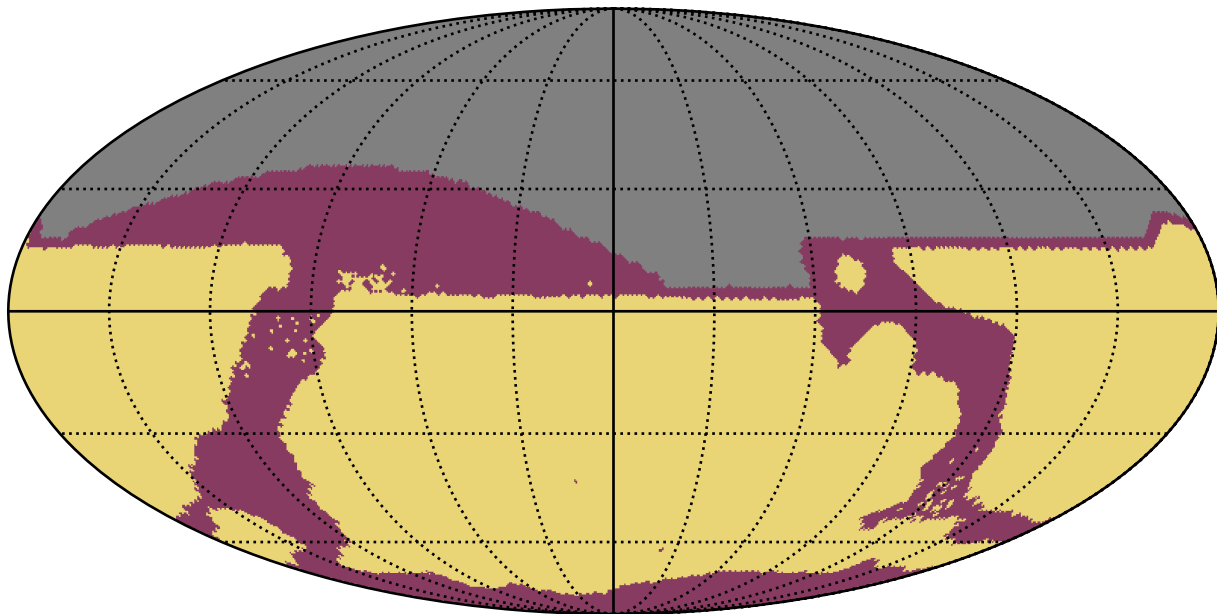
noroll_v3.4_10yrs All sky: RapidRevisits
