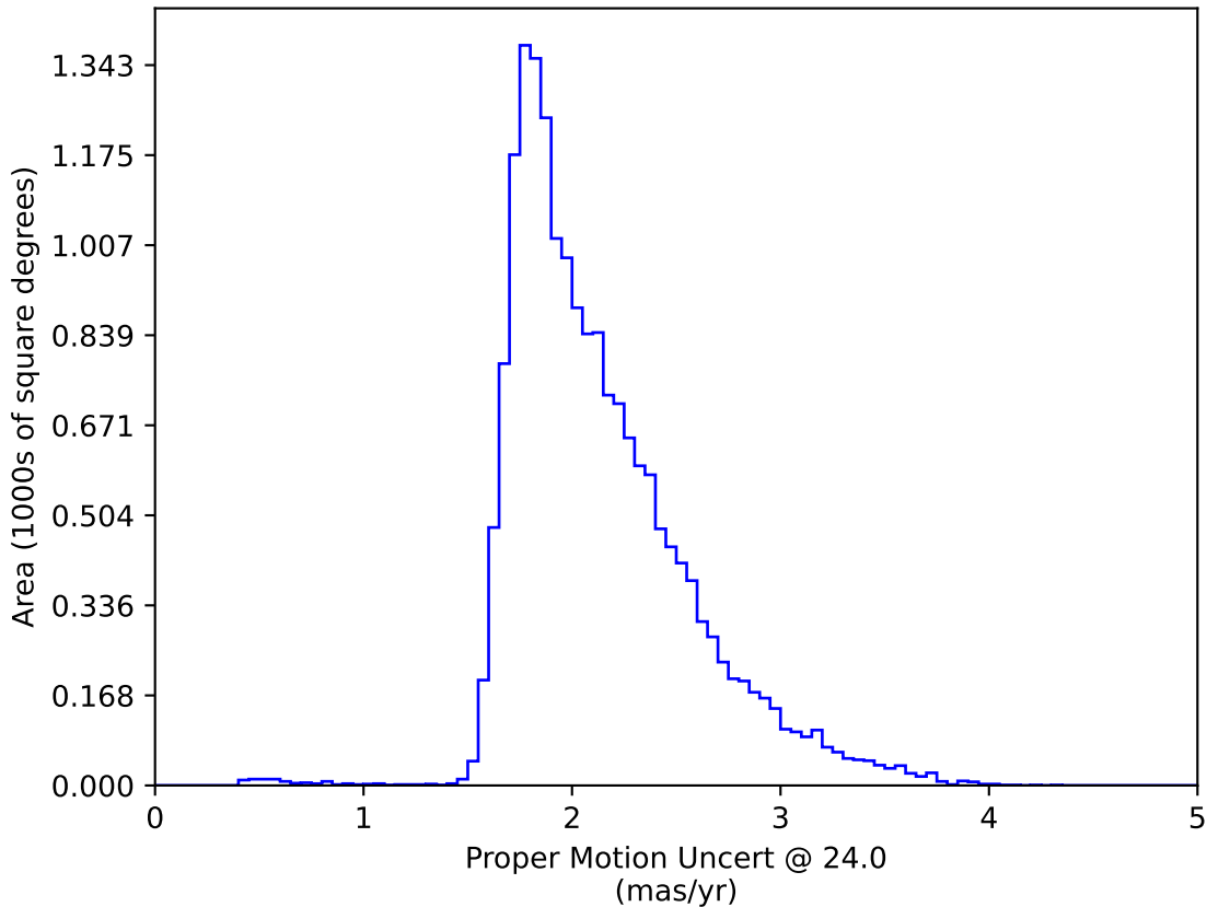
noroll_v3.4_10yrs WFD: Proper Motion Uncert @ 24.0
