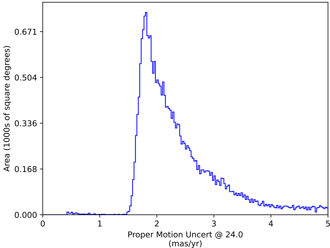
noroll_v3.4_10yrs All sky: Proper Motion Uncert @ 24.0
