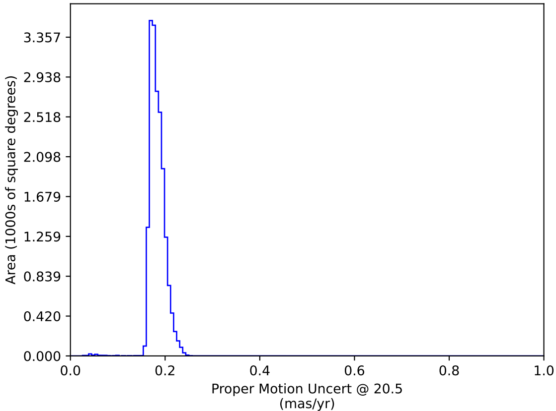
noroll_v3.4_10yrs WFD: Proper Motion Uncert @ 20.5
