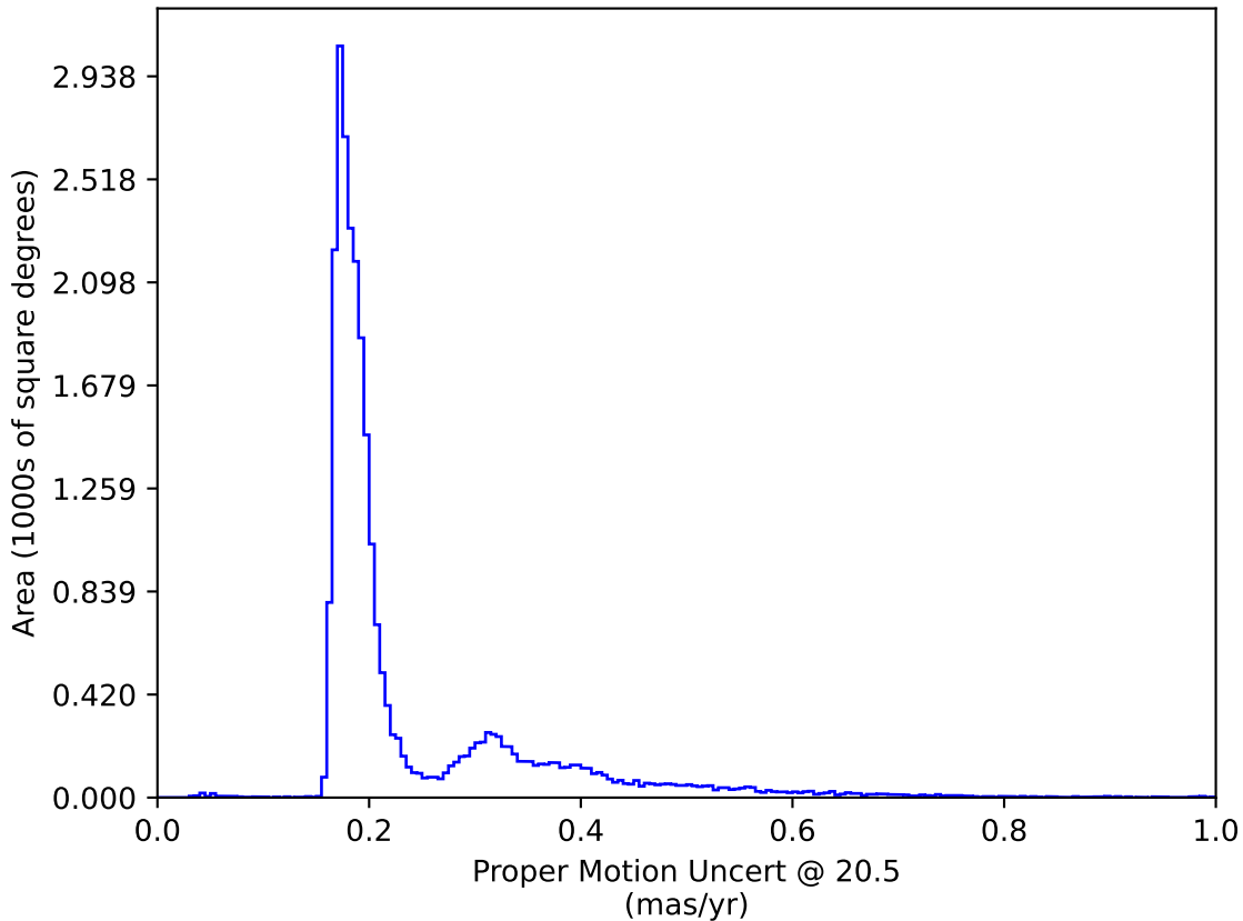
noroll_v3.4_10yrs All sky: Proper Motion Uncert @ 20.5
