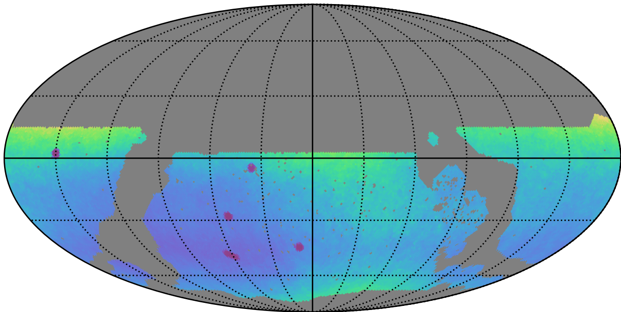
noroll_v3.4_10yrs WFD: Parallax Uncert @ 24.0
