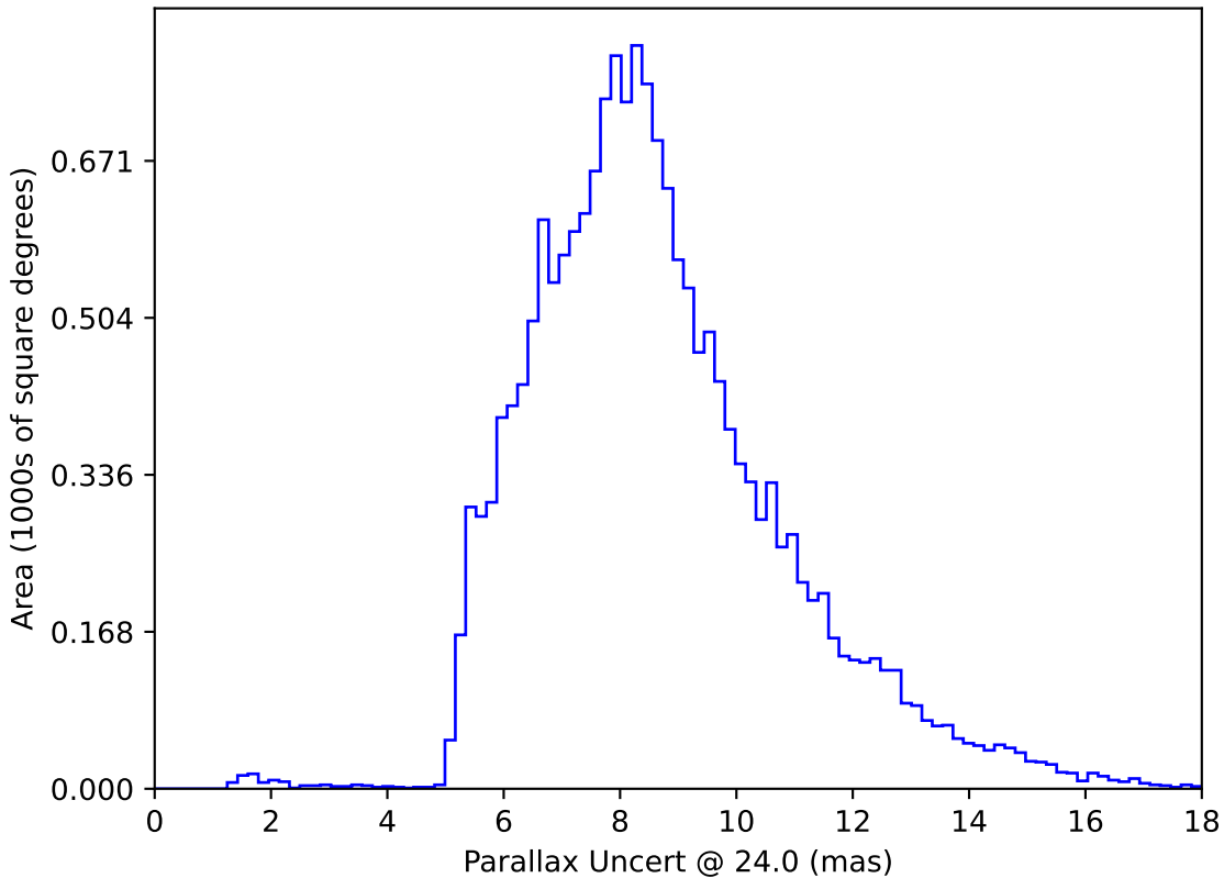
noroll_v3.4_10yrs WFD: Parallax Uncert @ 24.0
