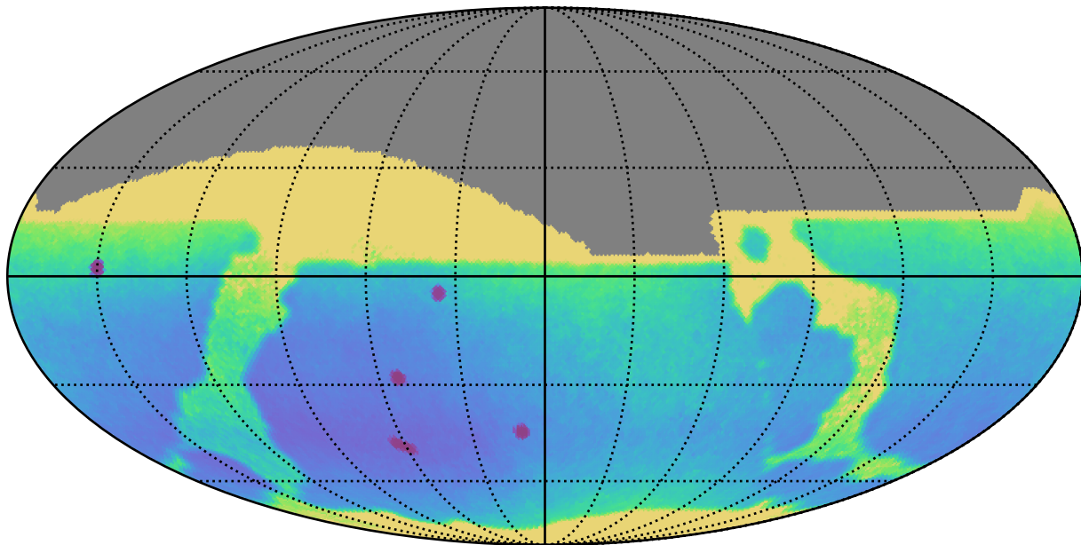
noroll_v3.4_10yrs All sky: Parallax Uncert @ 24.0
