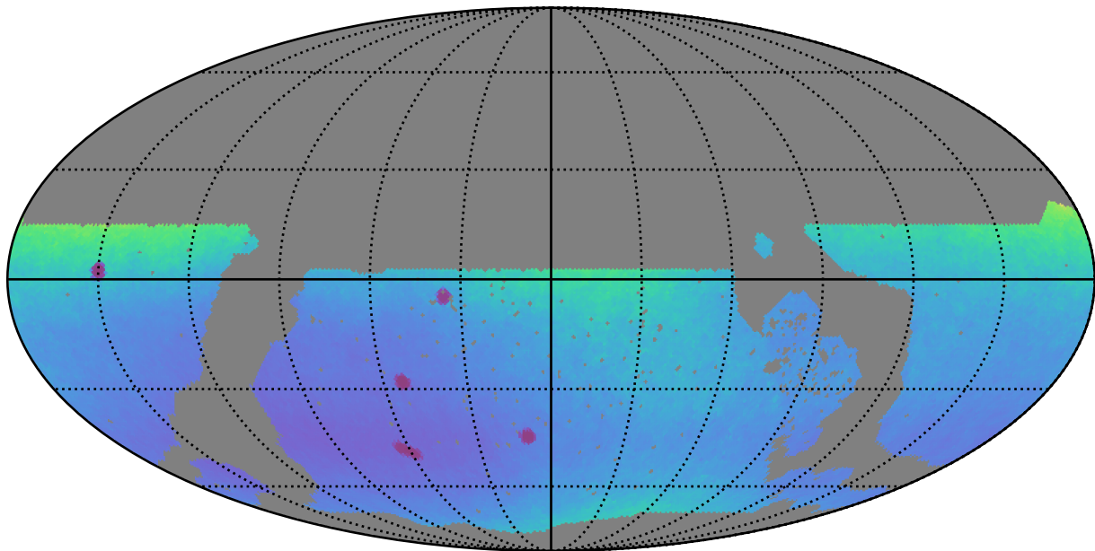
noroll_v3.4_10yrs WFD: Parallax Uncert @ 22.4
