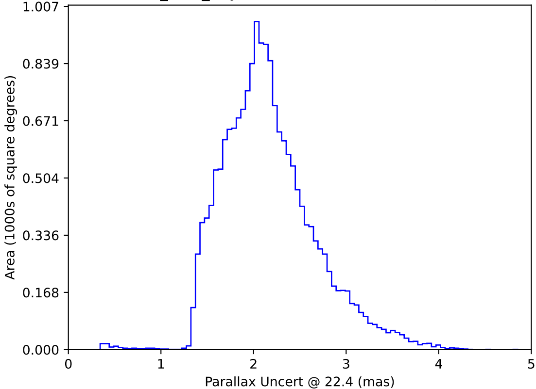
noroll_v3.4_10yrs WFD: Parallax Uncert @ 22.4
