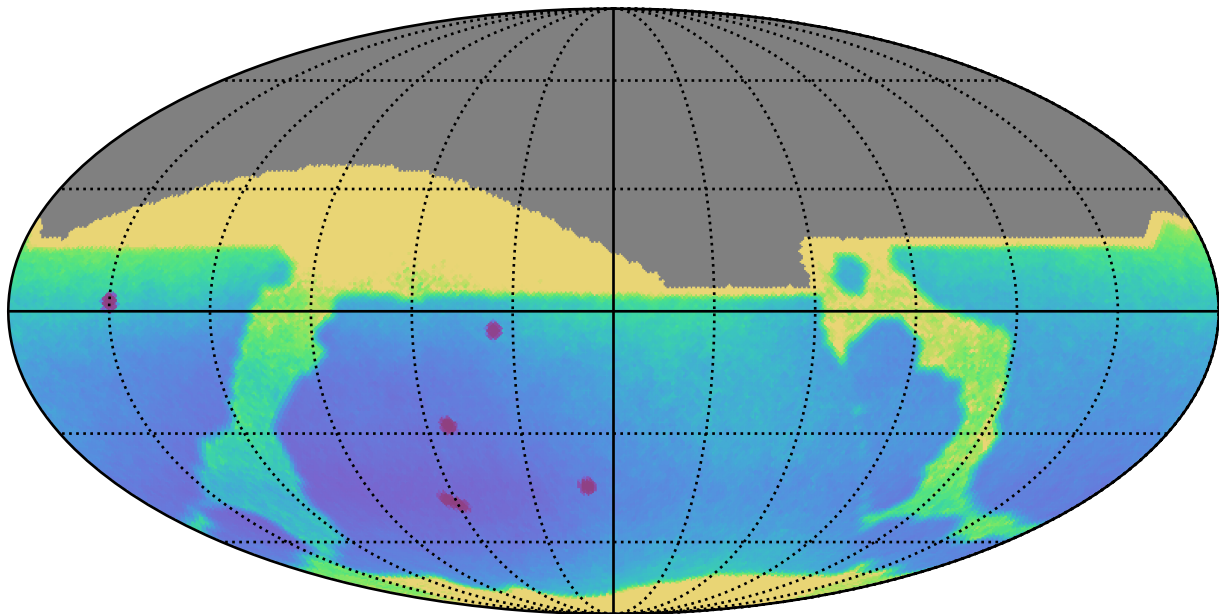
noroll_v3.4_10yrs All sky: Parallax Uncert @ 22.4
