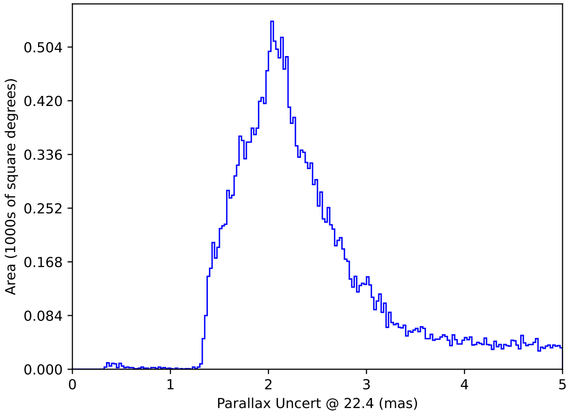
noroll_v3.4_10yrs All sky: Parallax Uncert @ 22.4
