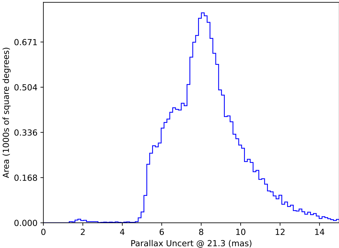
noroll_v3.4_10yrs WFD y band only: Parallax Uncert @ 21.3
