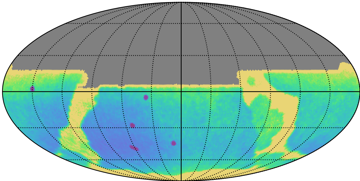
noroll_v3.4_10yrs All sky y band only: Parallax Uncert @ 21.3
