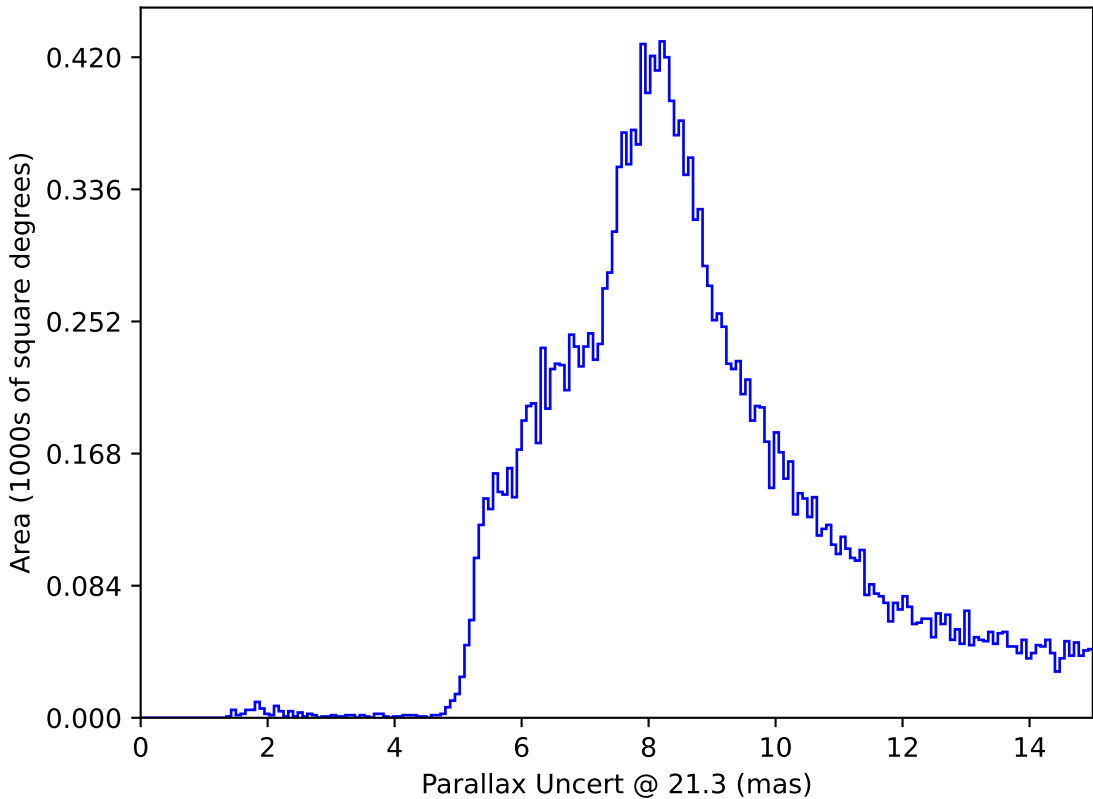
noroll_v3.4_10yrs All sky y band only: Parallax Uncert @ 21.3
