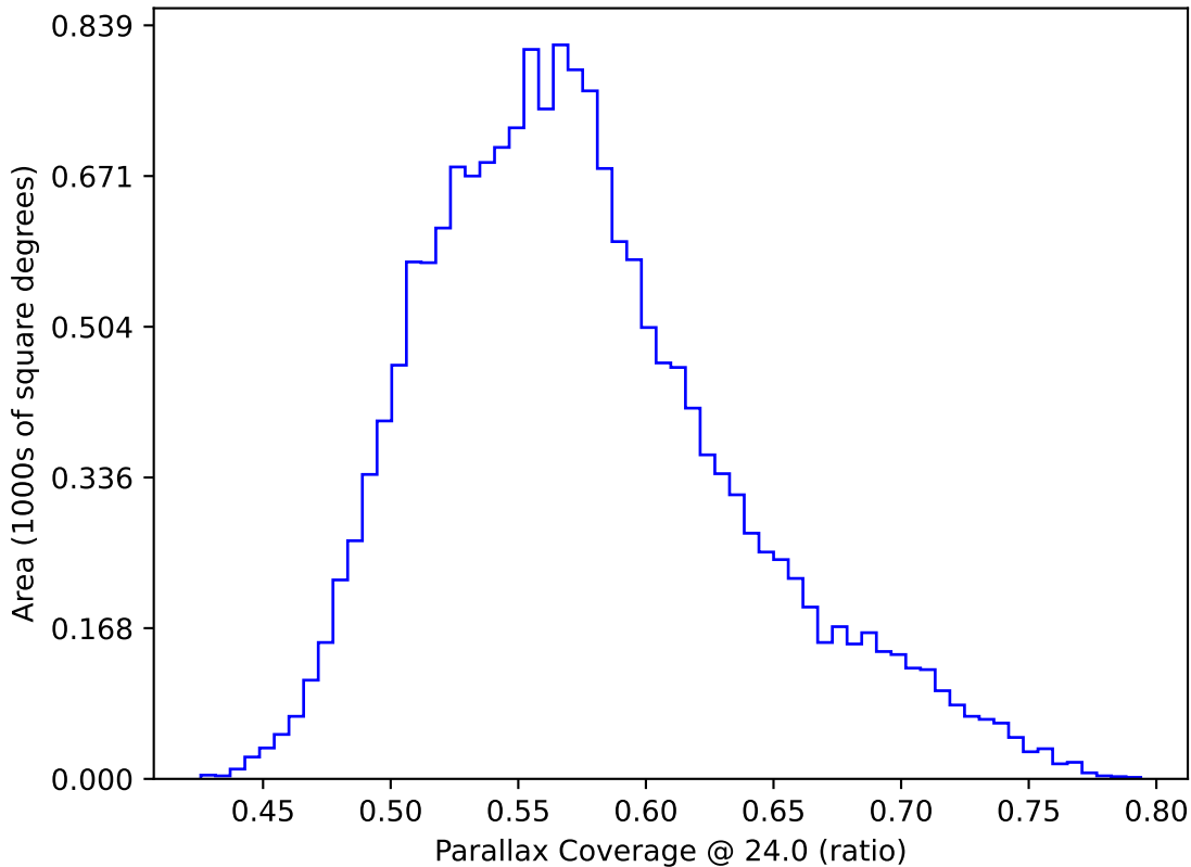
noroll_v3.4_10yrs WFD: Parallax Coverage @ 24.0
