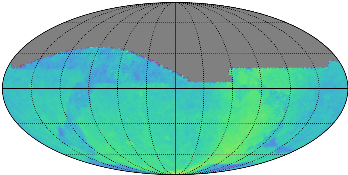
noroll_v3.4_10yrs All sky: Parallax Coverage @ 24.0
