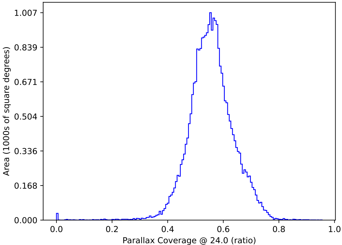
noroll_v3.4_10yrs All sky: Parallax Coverage @ 24.0
