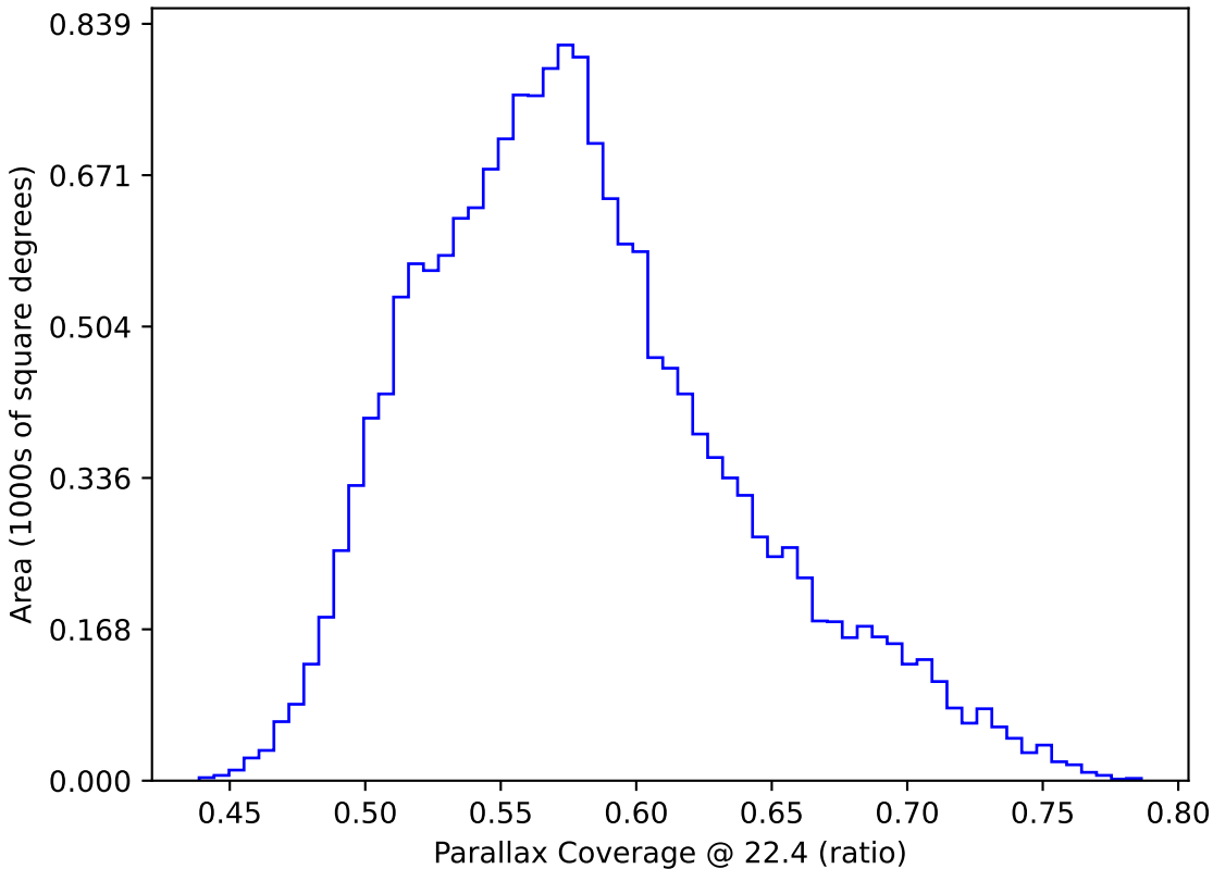
noroll_v3.4_10yrs WFD: Parallax Coverage @ 22.4
