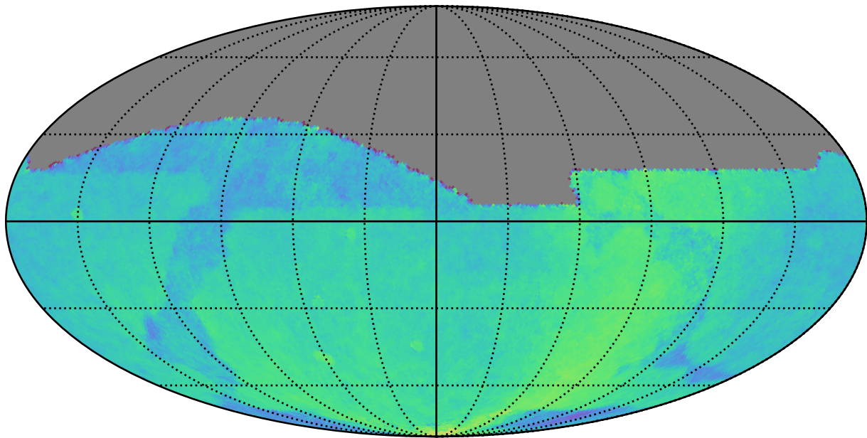
noroll_v3.4_10yrs All sky: Parallax Coverage @ 22.4
