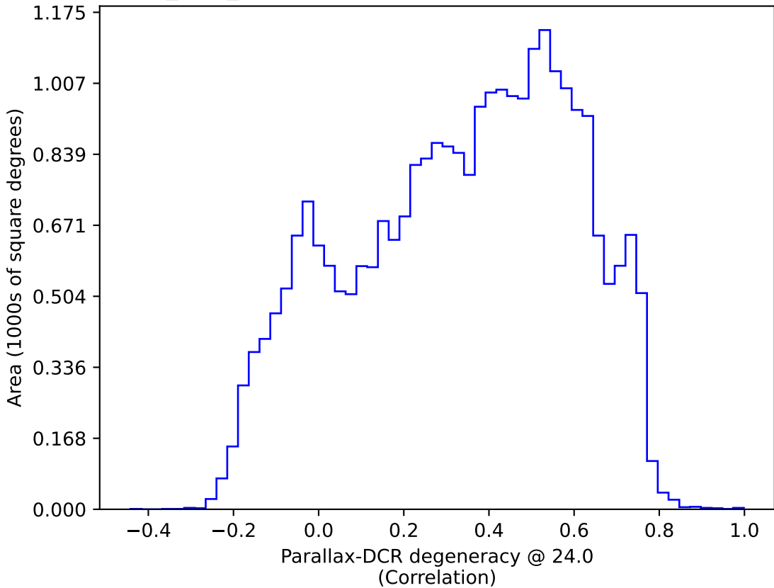
noroll_v3.4_10yrs All sky: Parallax-DCR degeneracy @ 24.0
