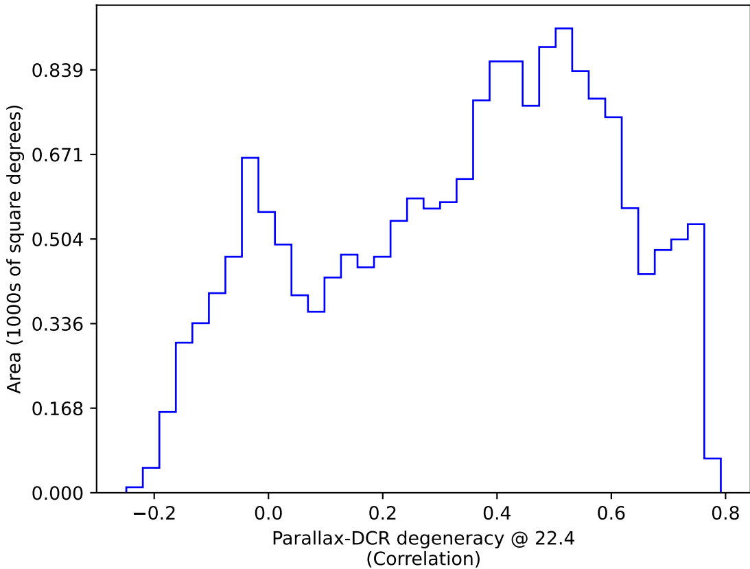
noroll_v3.4_10yrs WFD: Parallax-DCR degeneracy @ 22.4
