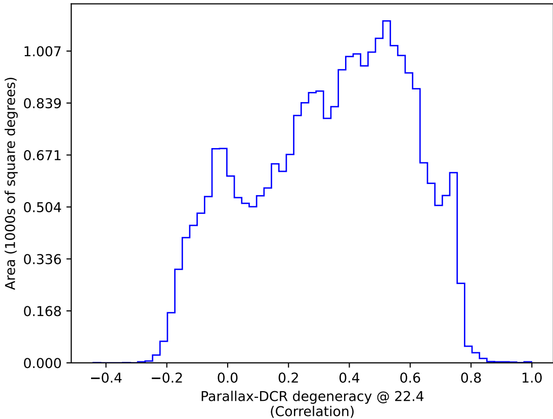
noroll_v3.4_10yrs All sky: Parallax-DCR degeneracy @ 22.4
