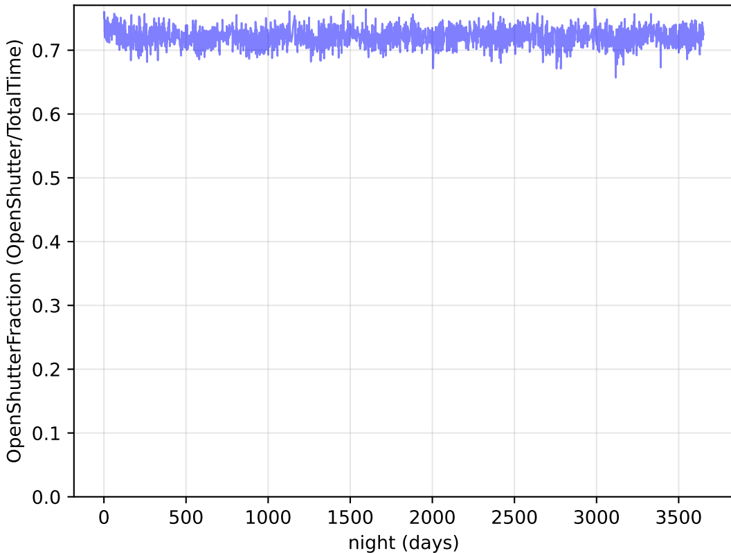
noroll_v3.4_10yrs Per night: OpenShutterFraction
