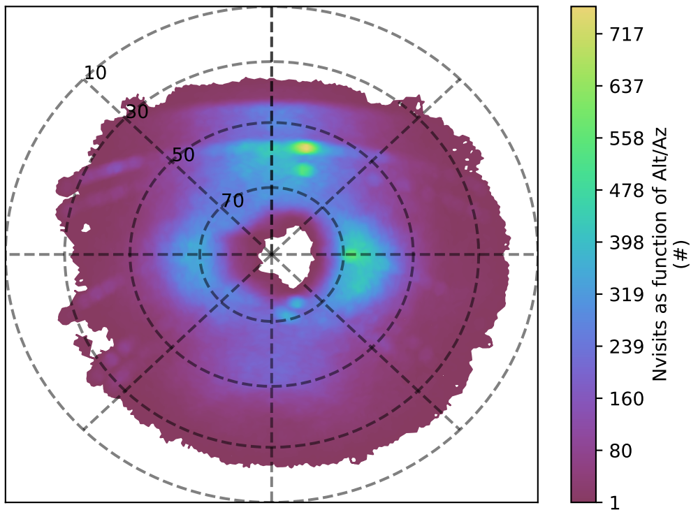
noroll_v3.4_10yrs u band: Nvisits as function of Alt/Az
