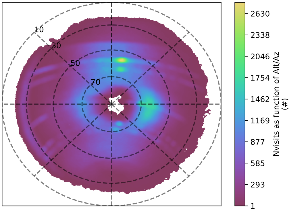
noroll_v3.4_10yrs r band: Nvisits as function of Alt/Az
