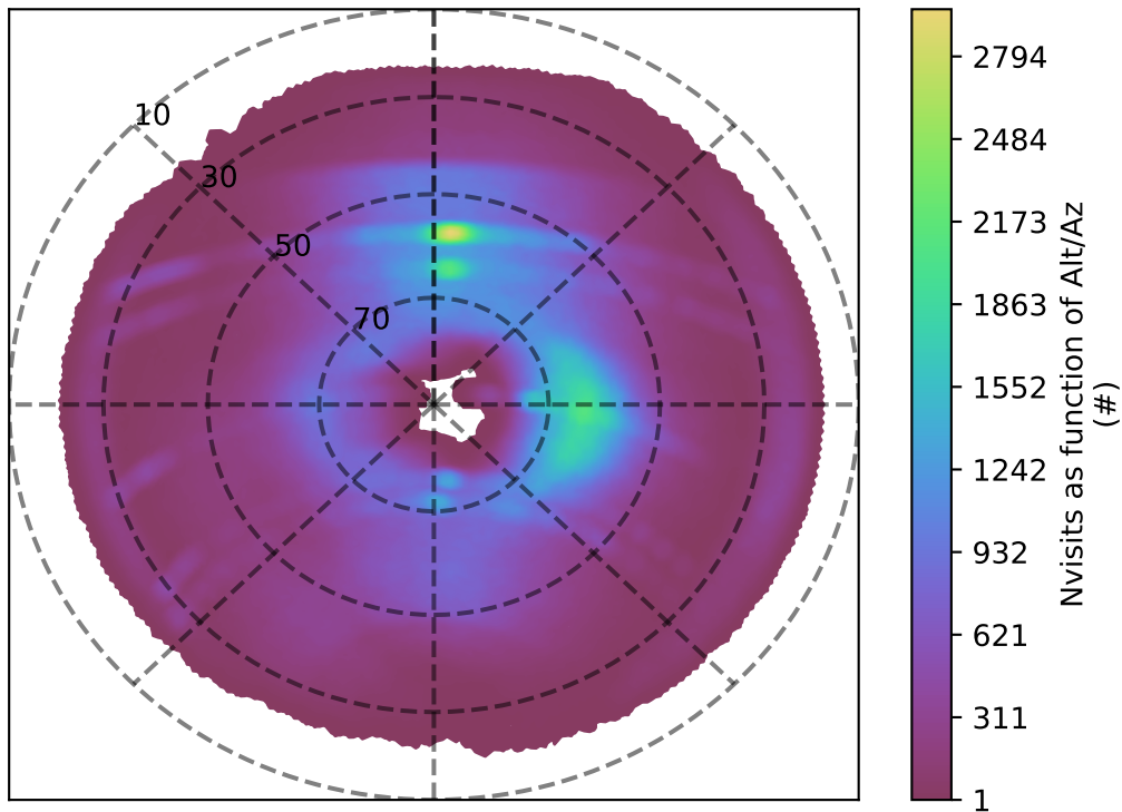
noroll_v3.4_10yrs i band: Nvisits as function of Alt/Az
