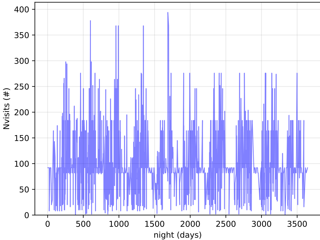
noroll_v3.4_10yrs DDF: Nvisits
