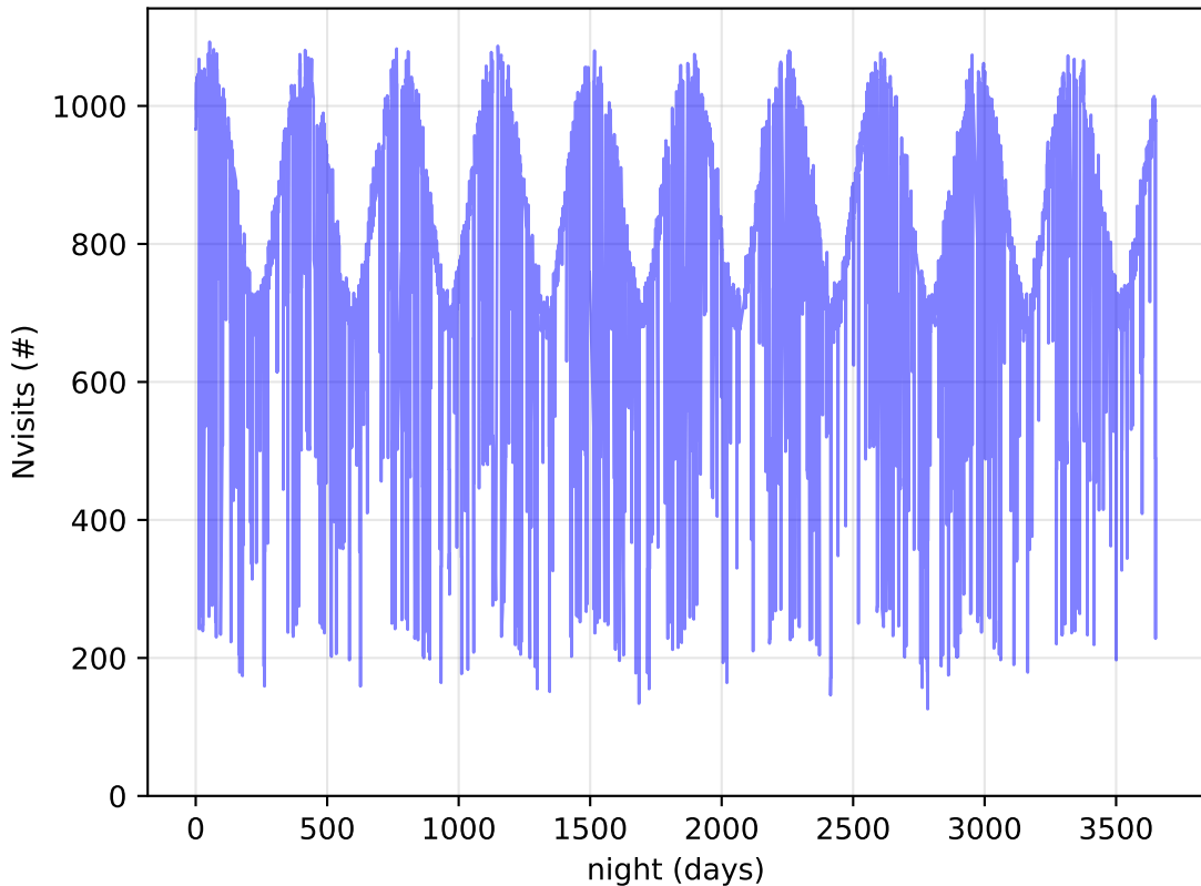
noroll_v3.4_10yrs All visits: Nvisits
