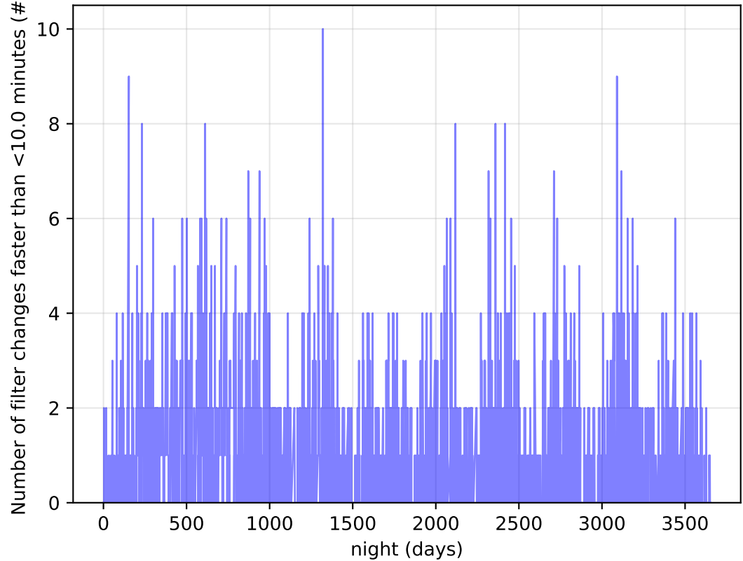
noroll_v3.4_10yrs Per Night: Number of filter changes faster than <10.0 minutes
