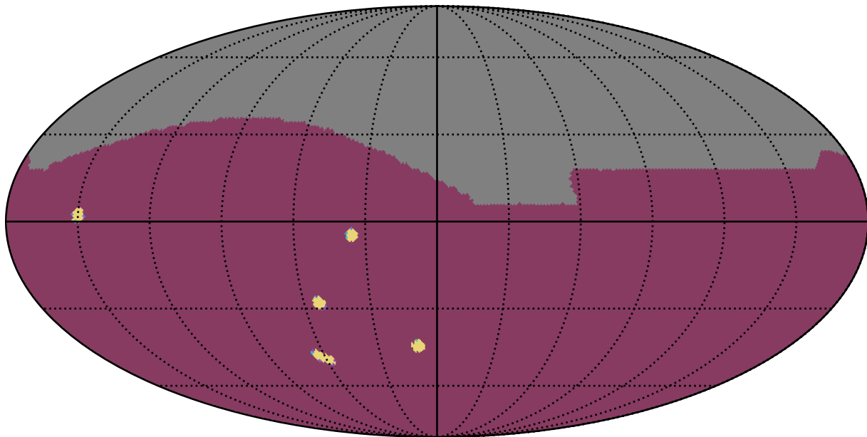
noroll_v3.4_10yrs All sky: NumberOfQuickRevisits
