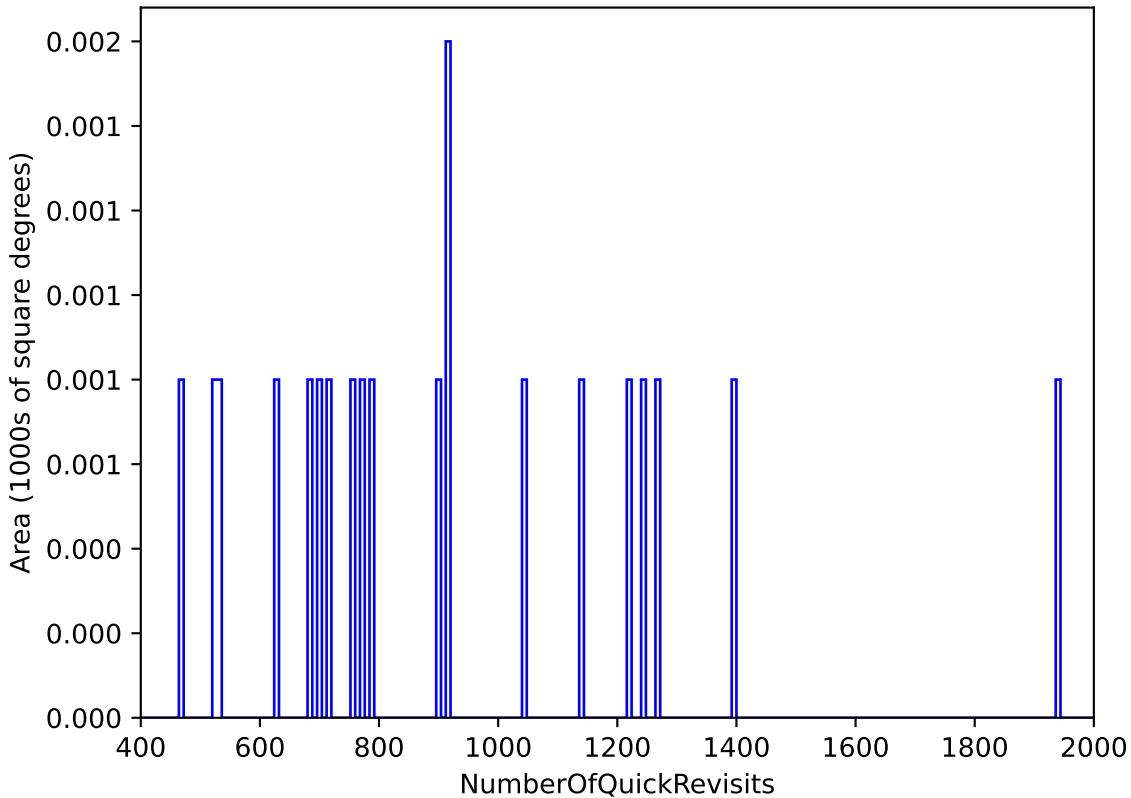
noroll_v3.4_10yrs All sky: NumberOfQuickRevisits
