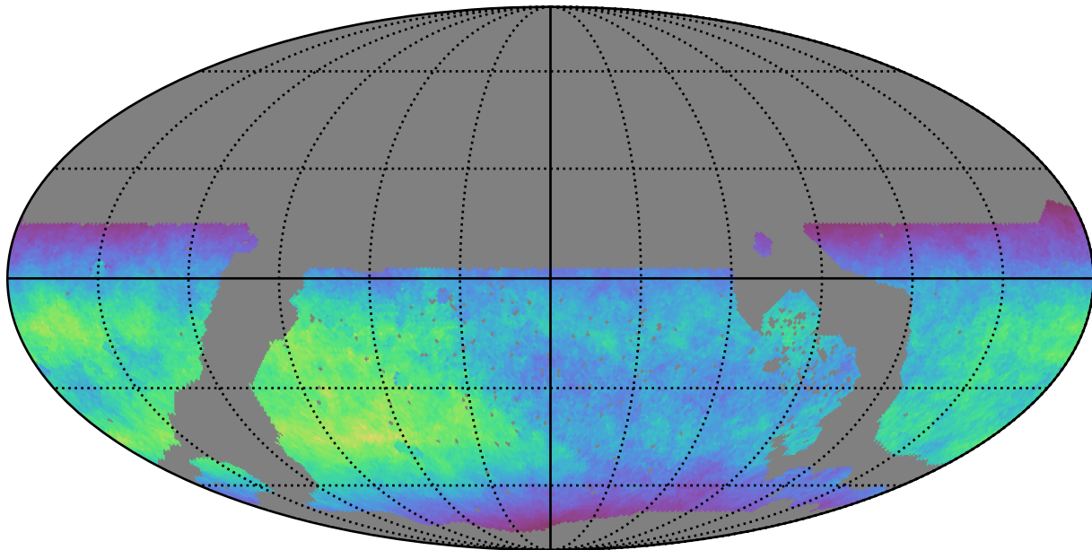
noroll_v3.4_10yrs WFD z band: Normalized Teff
