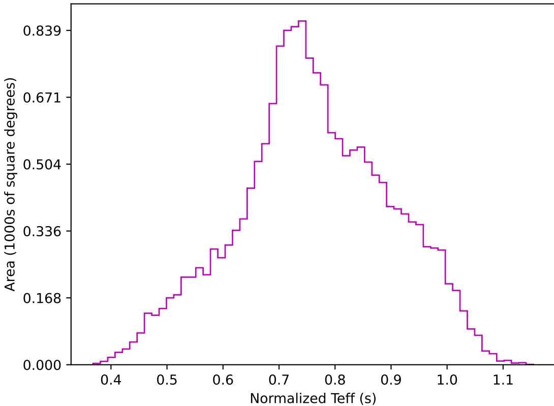
noroll_v3.4_10yrs WFD z band: Normalized Teff
