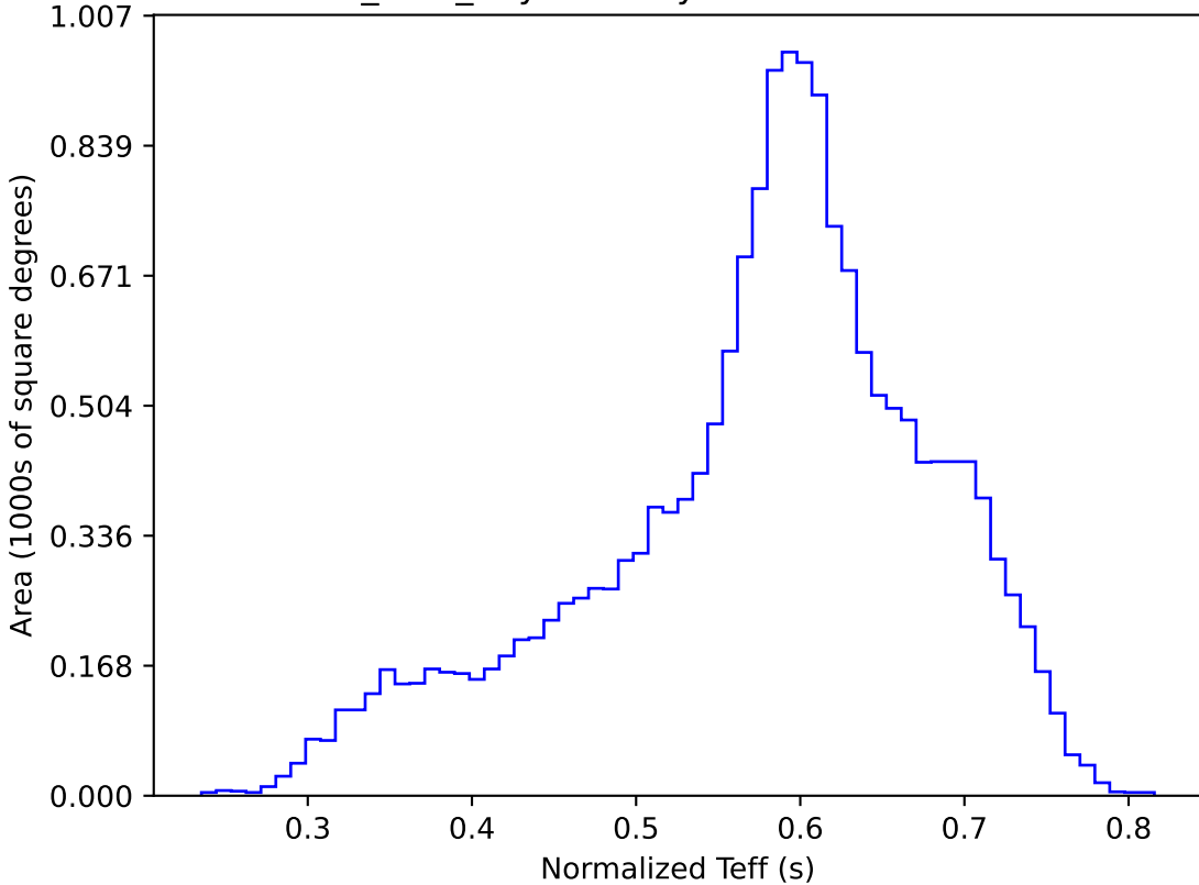
noroll_v3.4_10yrs WFD y band: Normalized Teff
