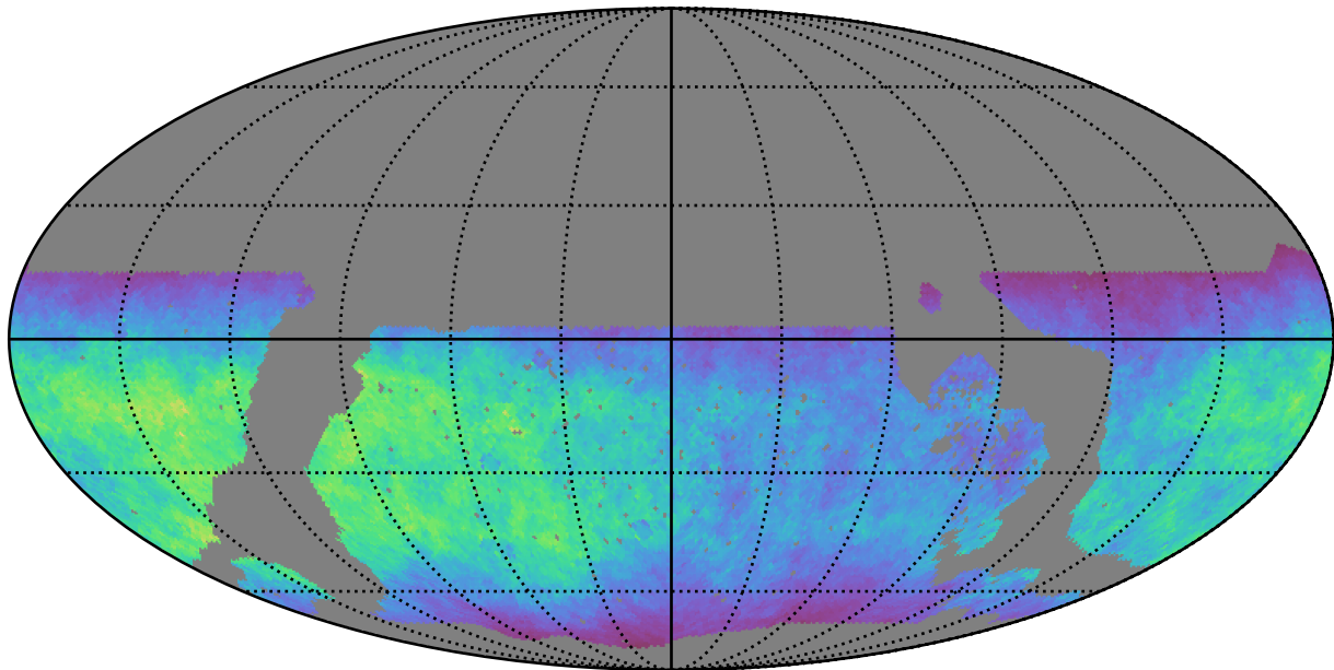
noroll_v3.4_10yrs WFD u band: Normalized Teff
