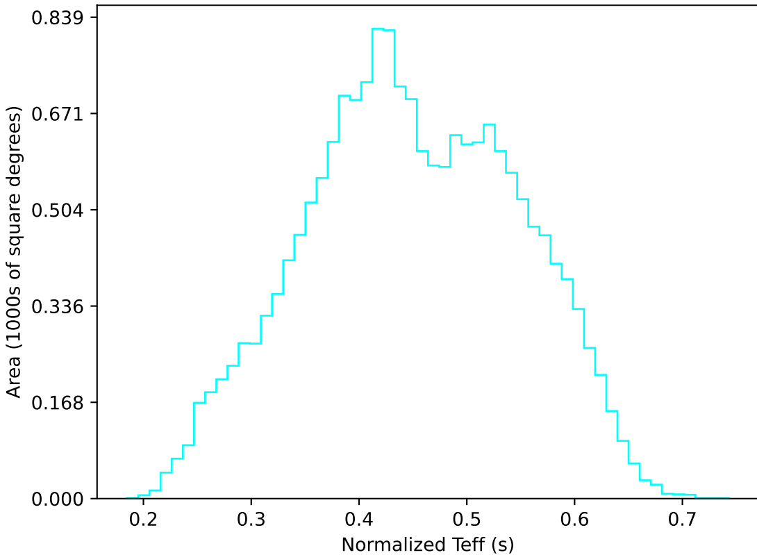
noroll_v3.4_10yrs WFD u band: Normalized Teff
