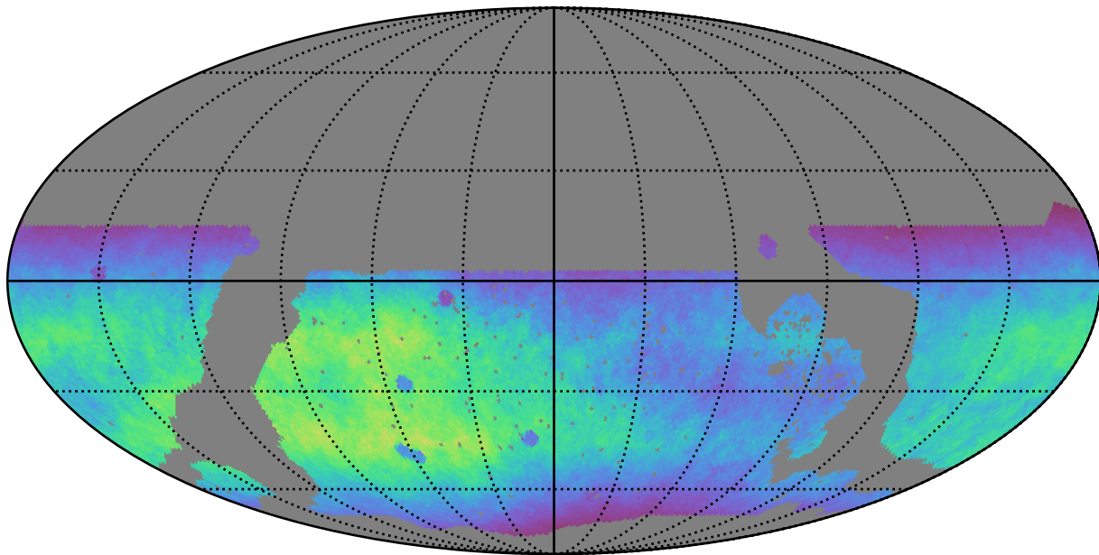
noroll_v3.4_10yrs WFD r band: Normalized Teff
