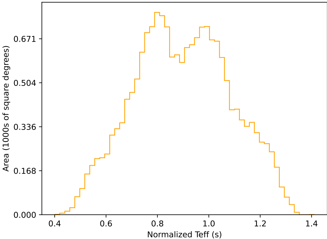
noroll_v3.4_10yrs WFD r band: Normalized Teff
