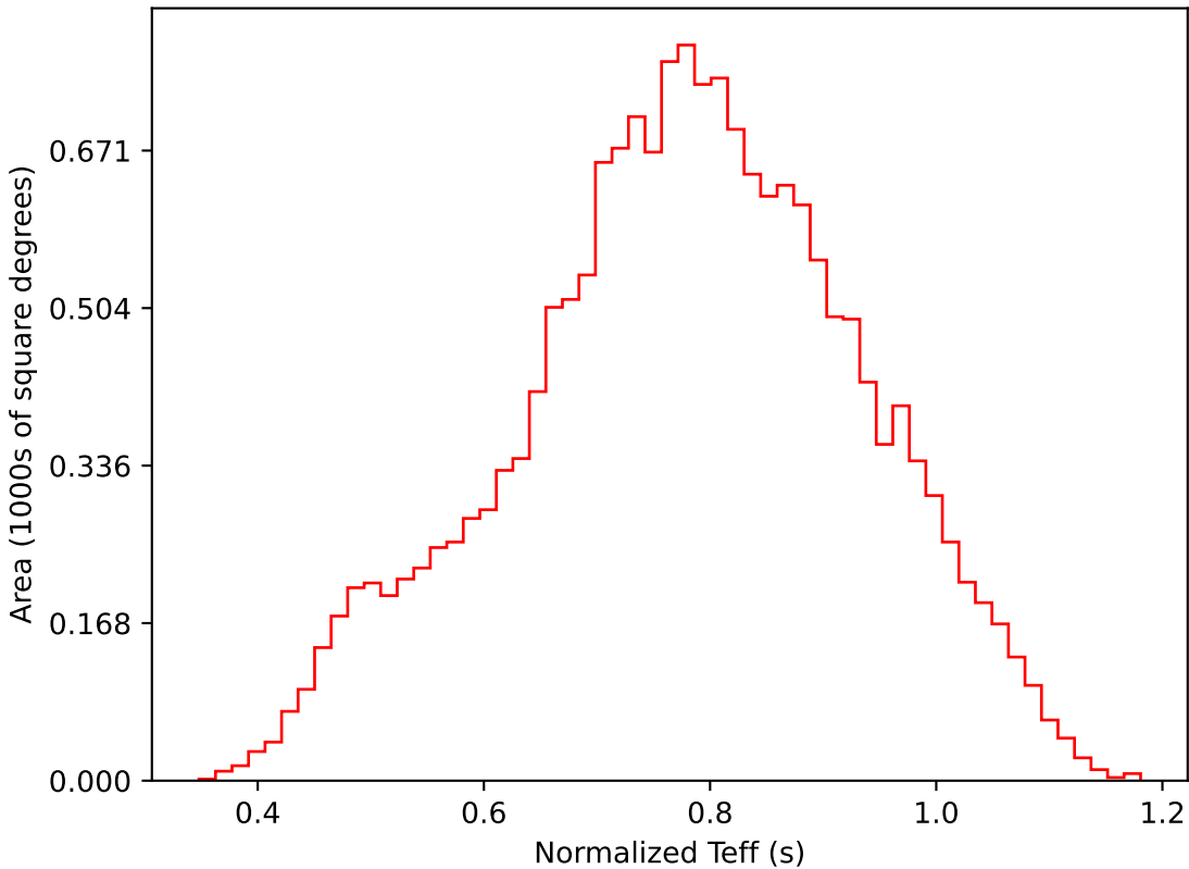
noroll_v3.4_10yrs WFD i band: Normalized Teff
