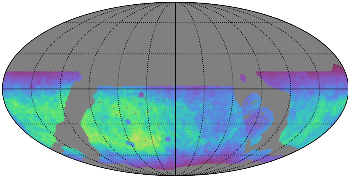
noroll_v3.4_10yrs WFD g band: Normalized Teff
