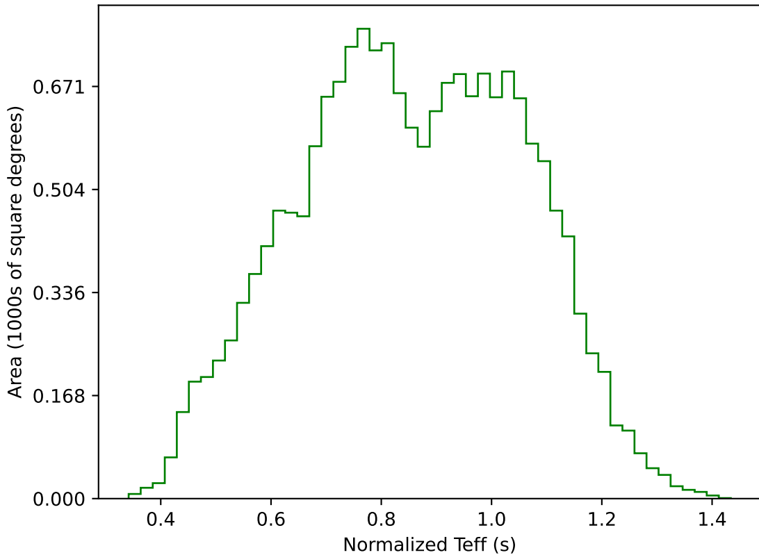
noroll_v3.4_10yrs WFD g band: Normalized Teff
