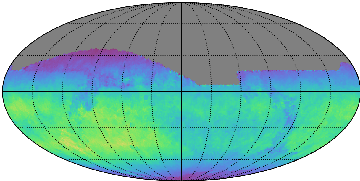
noroll_v3.4_10yrs All sky z band: Normalized Teff
