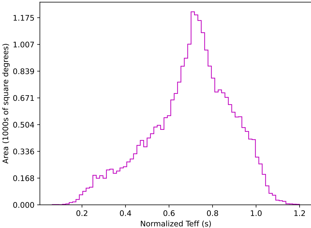
noroll_v3.4_10yrs All sky z band: Normalized Teff
