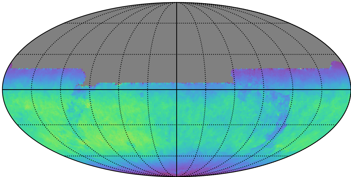
noroll_v3.4_10yrs All sky y band: Normalized Teff
